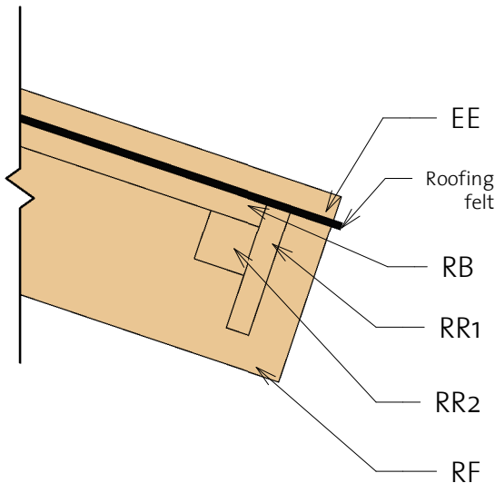
3) Roof Reinforcement
