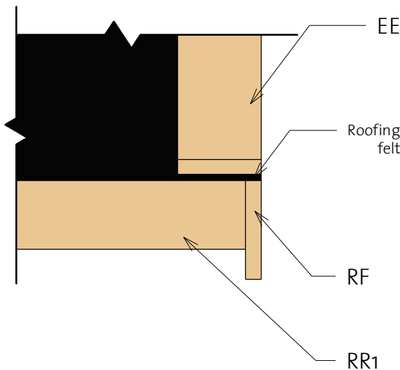
3) Roof Reinforcement
