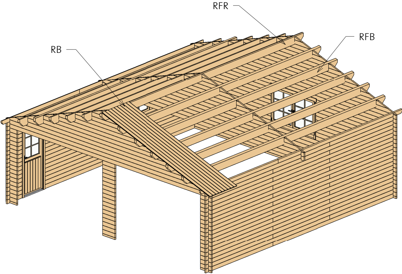
Roof 1
